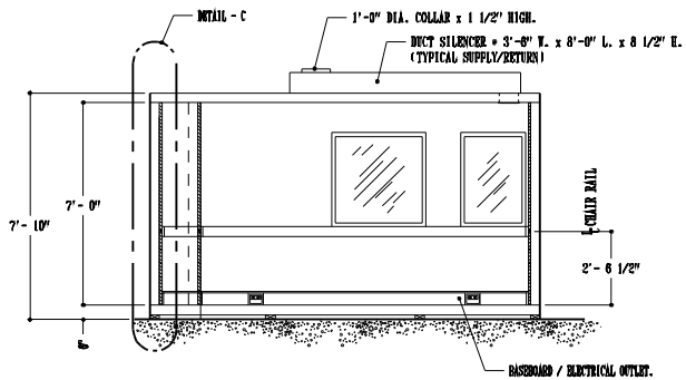
D WINDOW ELEVATION VIEW
