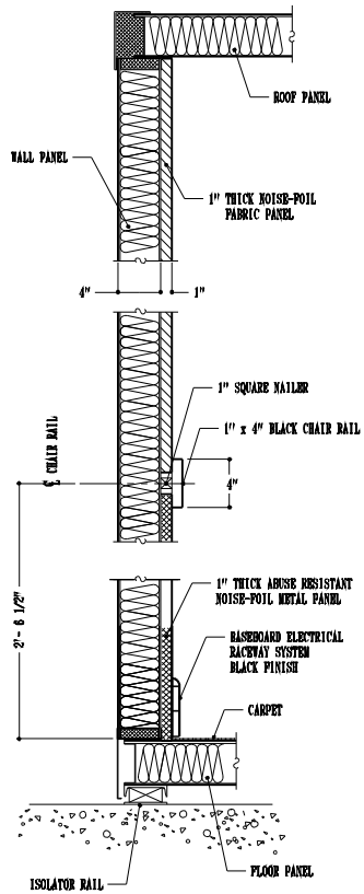
C ENHANCEMENT DETAIL
